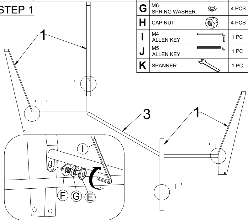
DETAIL I
